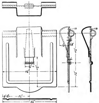
Figs. 4502-4506. Morris Pressed Steel Journal Box Lid.
